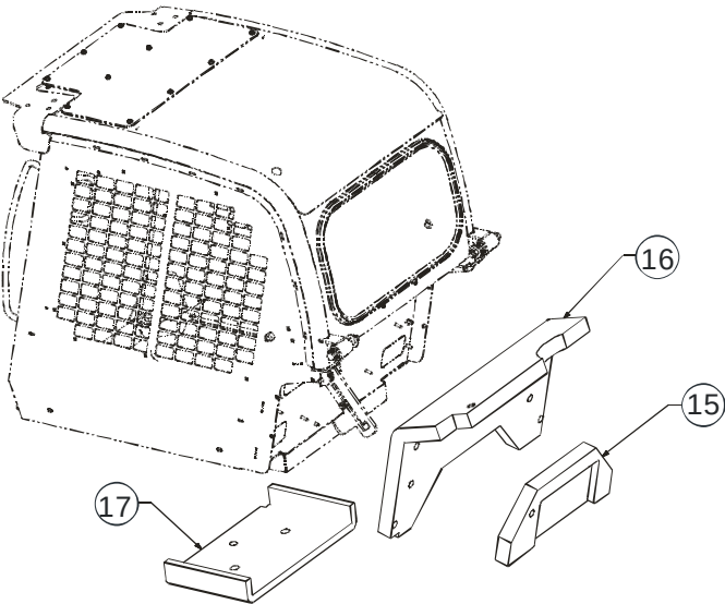
FRONT FLOOR ASSEMBLY
