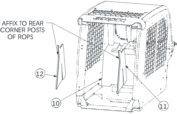
ROPS FRONTAL VIEW
