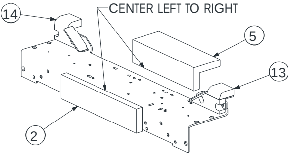
BOLTED-IN CROSSMEMBER
