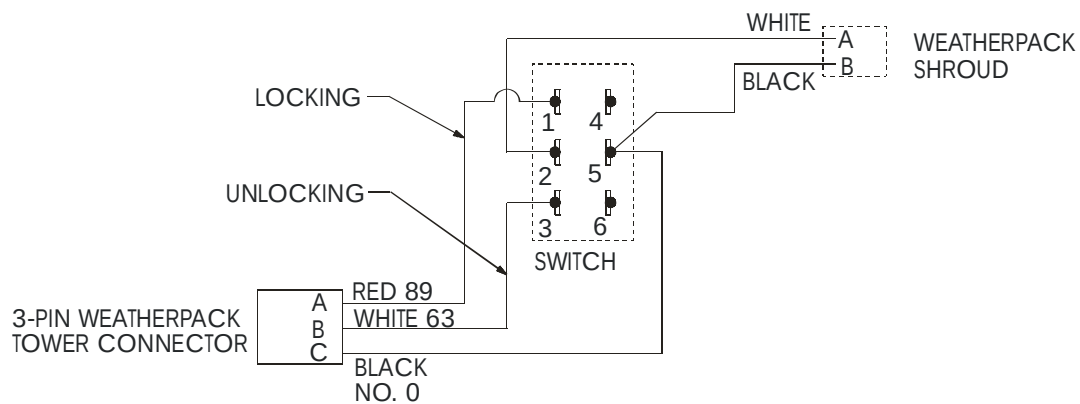
ELECTRICAL SCHEMATIC
