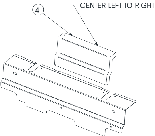
COVER/CONTROLS
