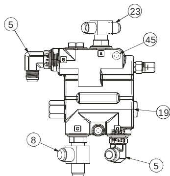
SELF-LEVELING VALVE DETAIL
