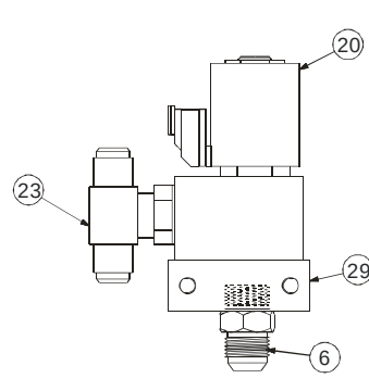
LIFT-LOCK SOLENOID
