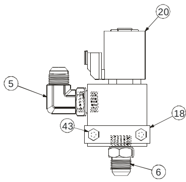
TILT-LOCK SOLENOID
